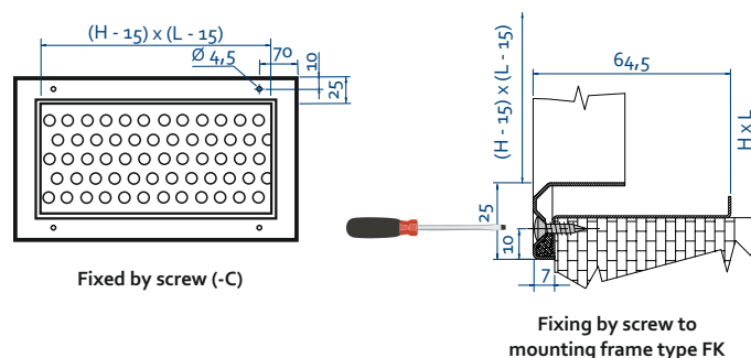
3. Installation of the grilles
