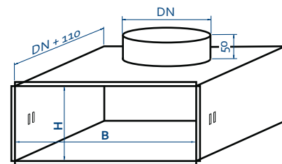
DLLS plenum box side connection
