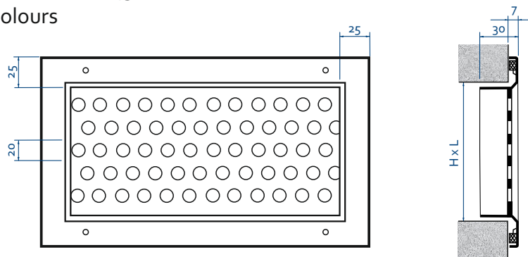
1. Dimensions of ventilation grilles type CNP
