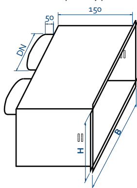
DLFS plenum box with top connection
